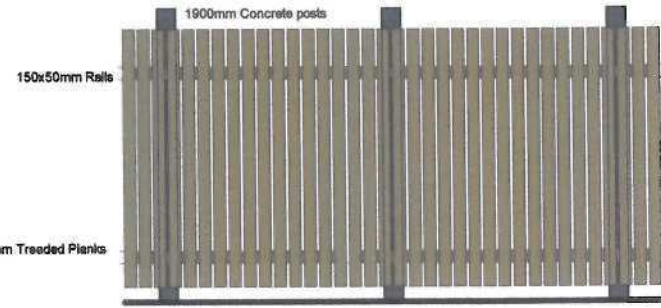
Fence Elevation Scale 1:50
